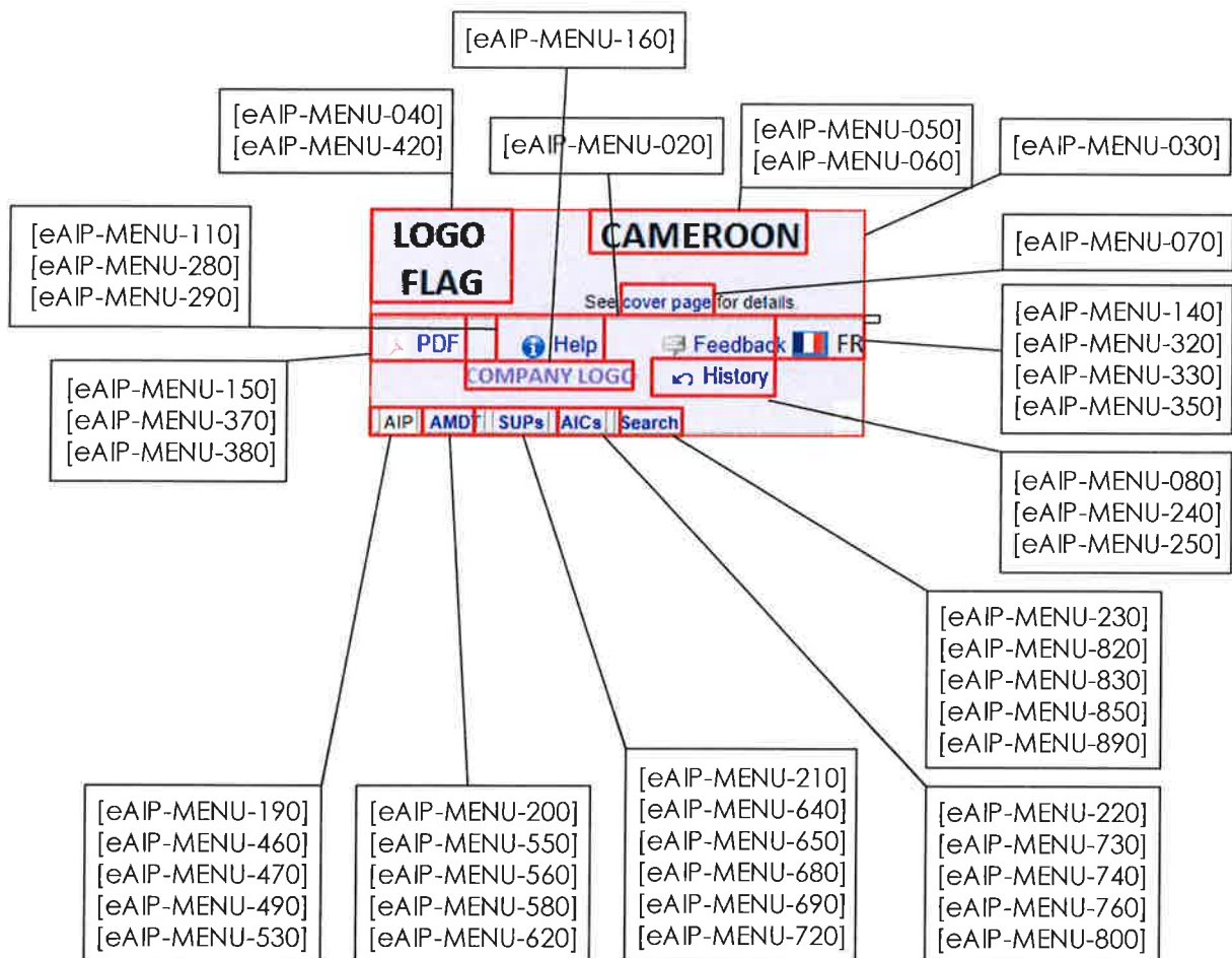
Figure 9: Commands Pane
