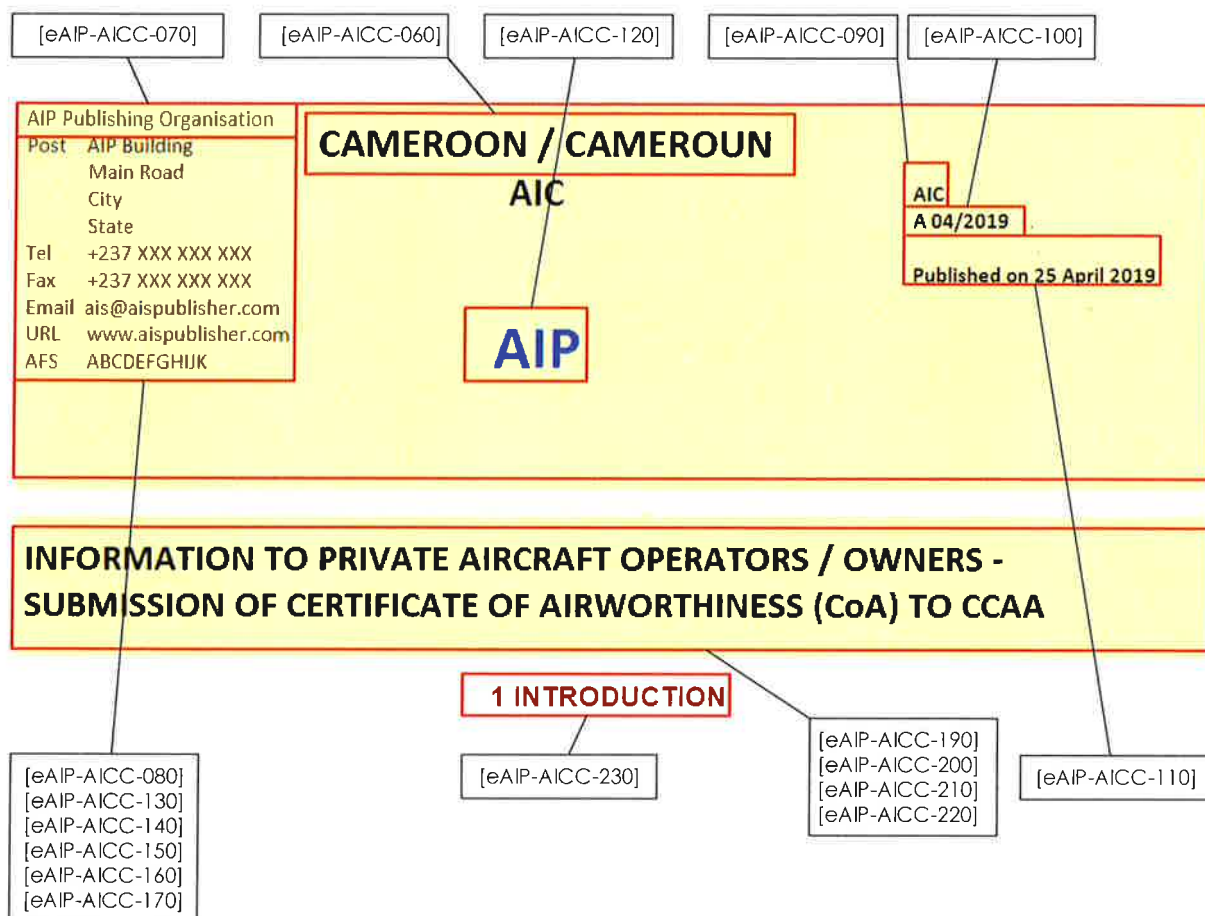
Figure 20: AIC Content
