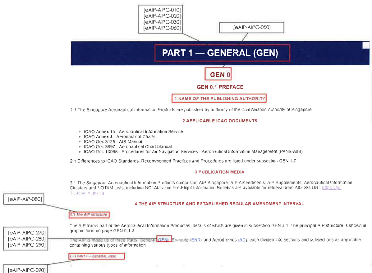
Figure 14: eAIP Content
