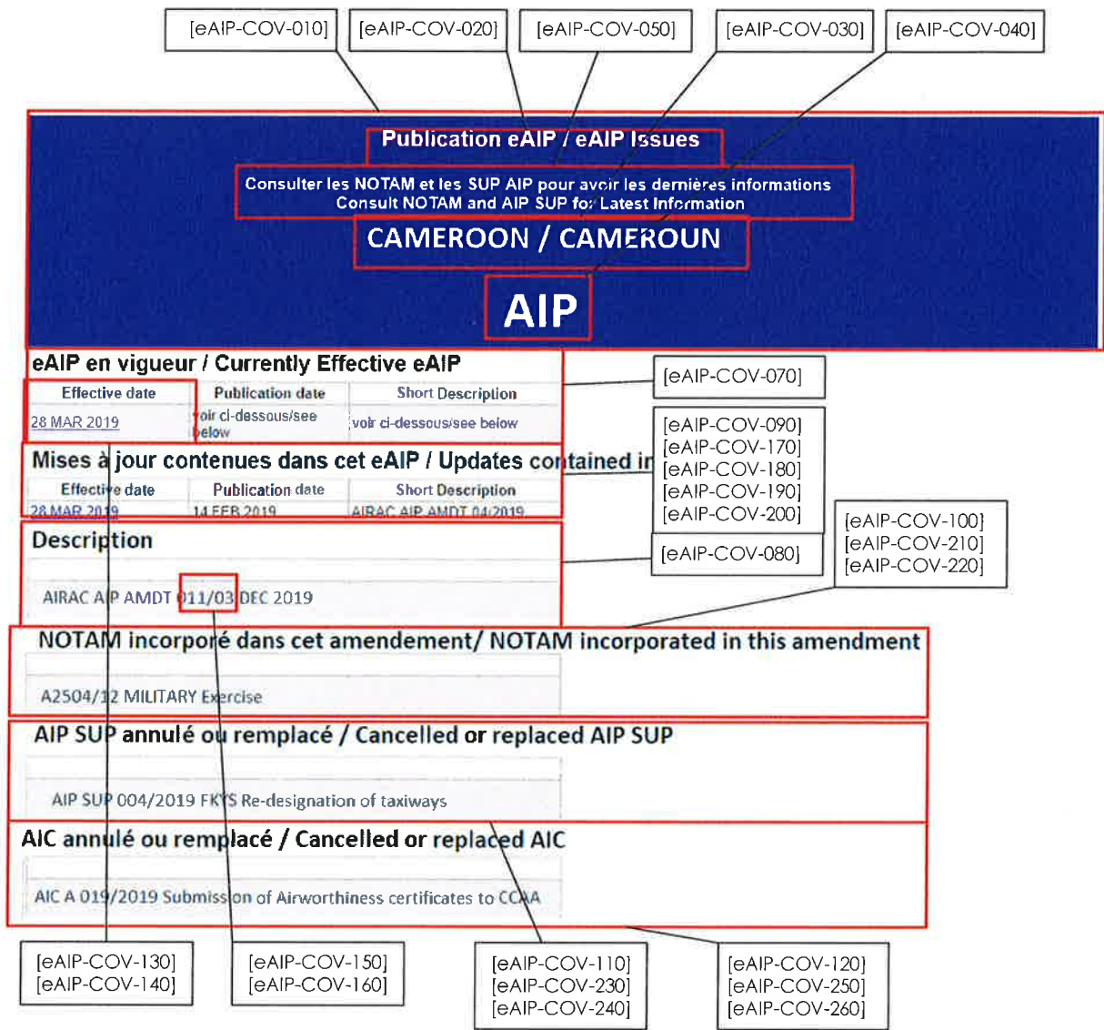
Figure 8: Cover Page
