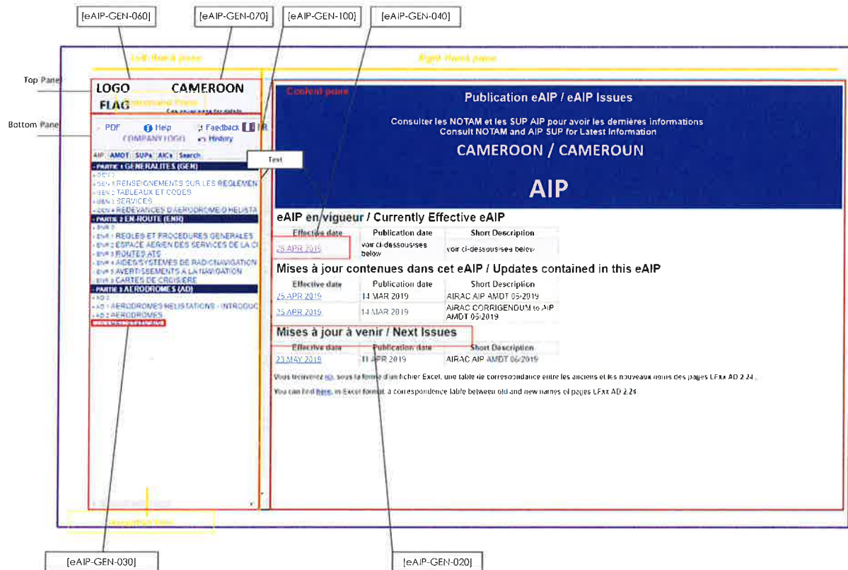
Figure 1: eAIP Window
